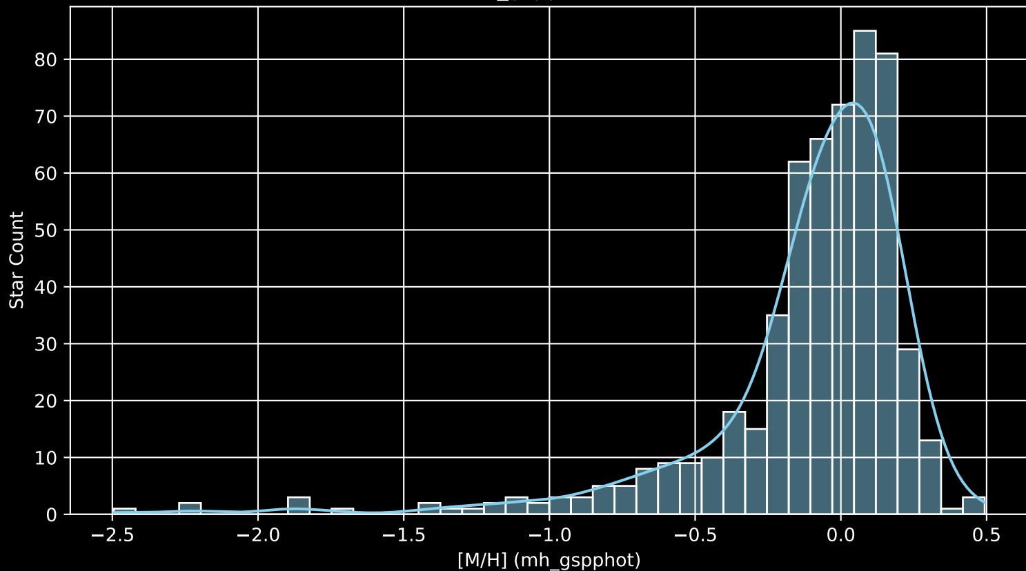
APOGEE DR17 Field: [300+04 [M/H] (mh_gspphot) (n= 550)
