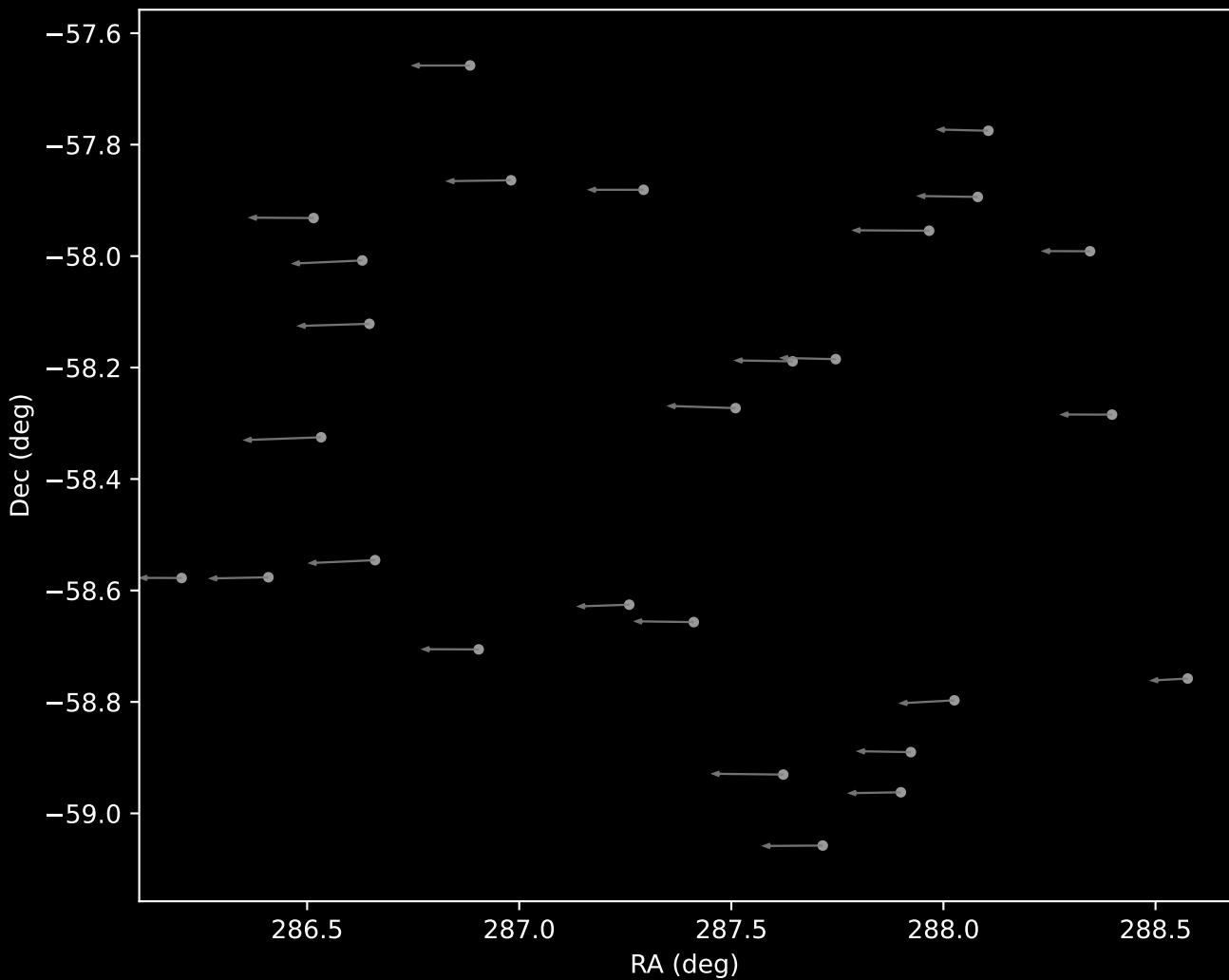
APOGEE DR17 Cluster 14 Proper Motion Vectors (n=27)
