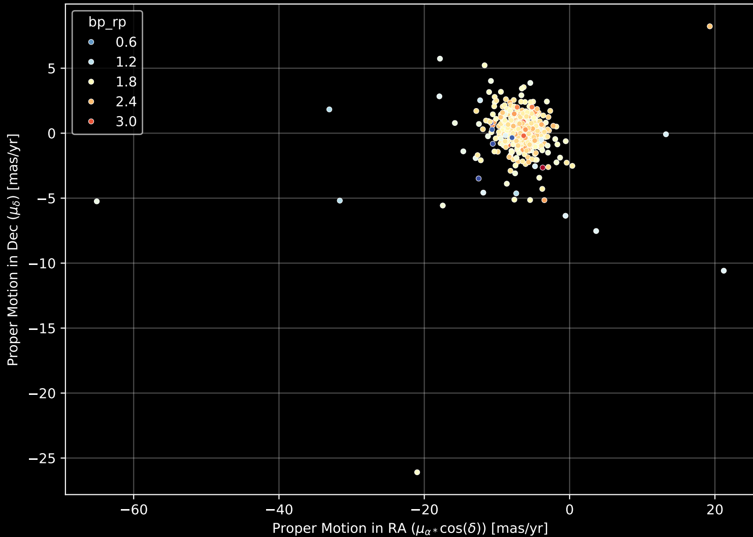
APOGEE DR17 Field: [300+04] Proper Motion Diagram (n= 554)
