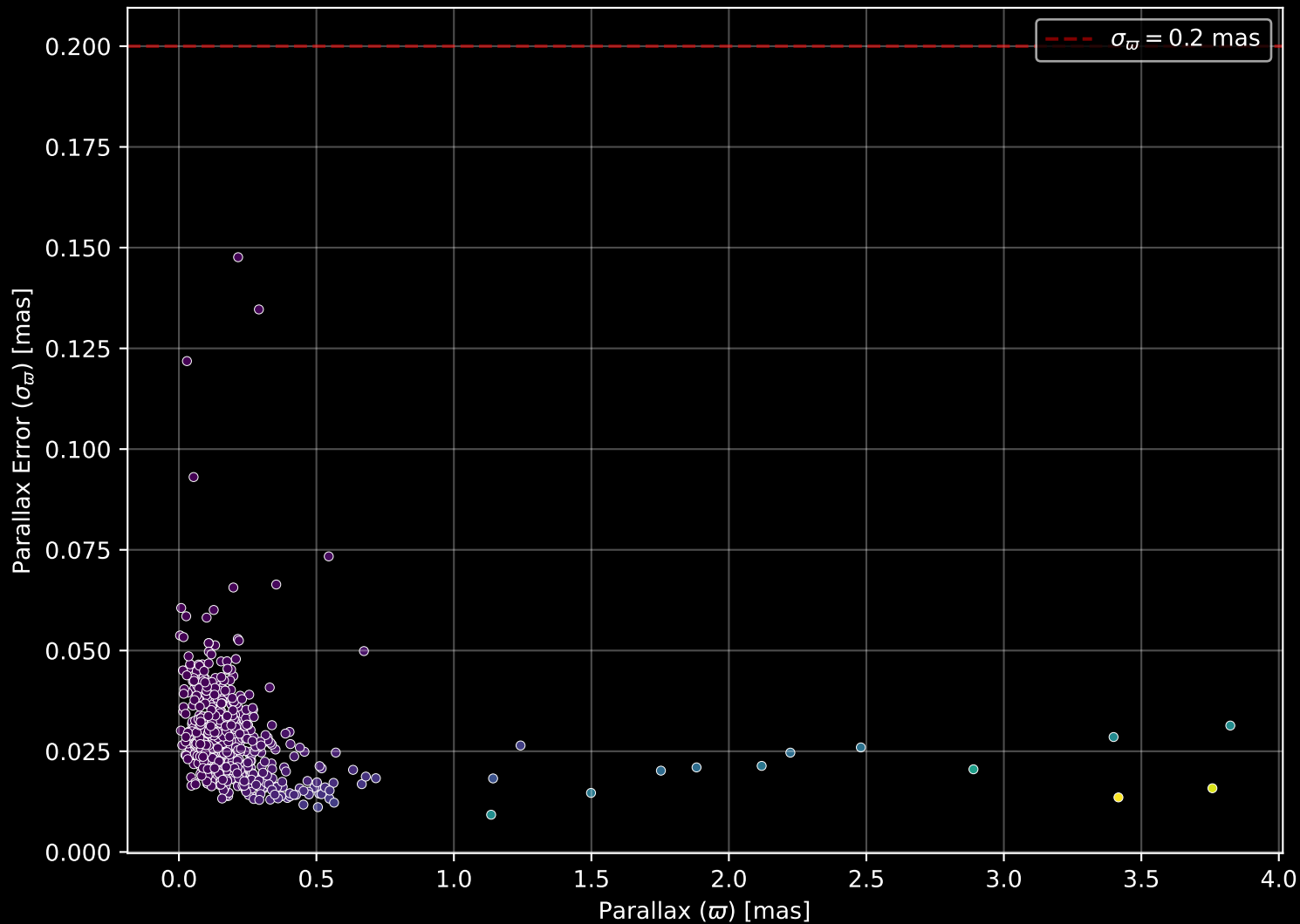
APOGEE DR17 Field: [300+04] Parallax Quality (n= 554)
