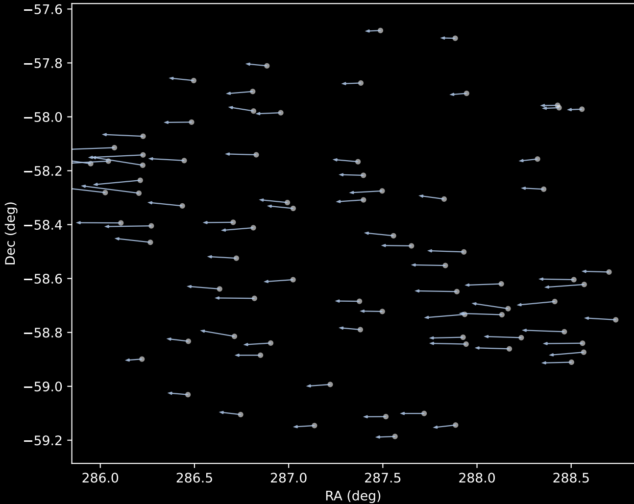
APOGEE DR17 Cluster 21 Proper Motion Vectors (n=81)
