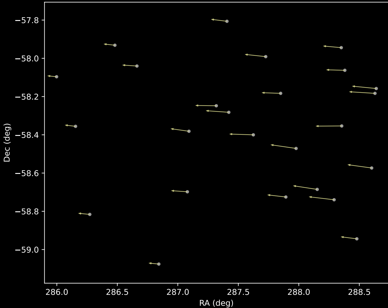
APOGEE DR17 Cluster 17 Proper Motion Vectors (n=25)
