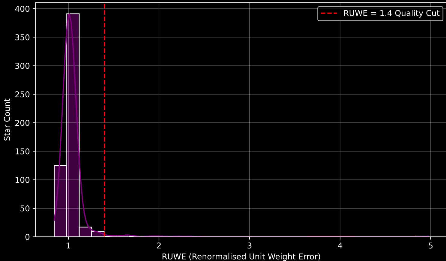
GAPOGEE DR17 Field [300+04] RUWE Distribution (n= 552)
