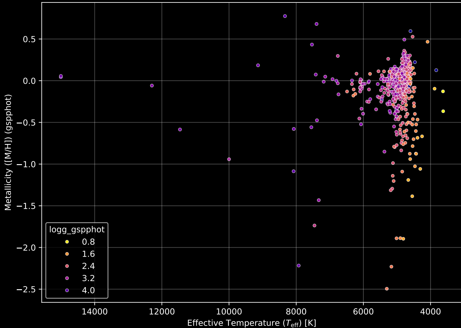
APOGEE DR17 Field: [300+04] Stellar Population Parameters (n= 554)
